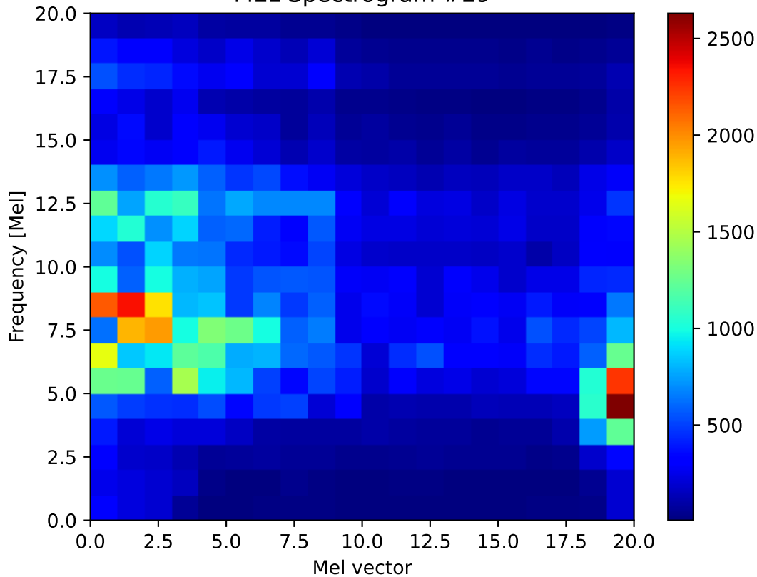
MEL Spectrogram #29
